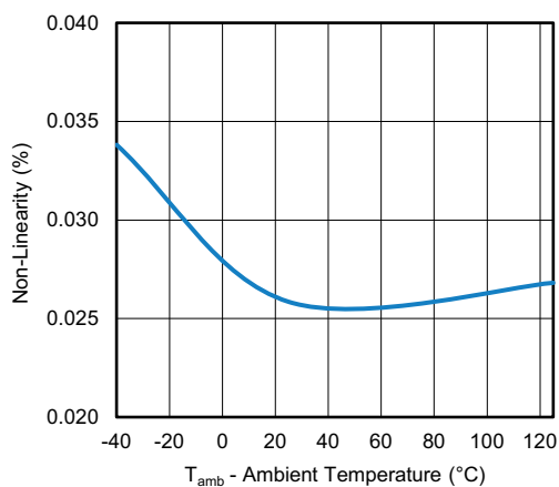
Fig. 8 - Non-Linearity vs. Ambient Temperature
