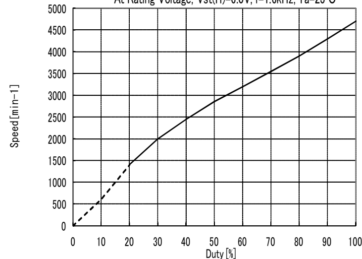
Duty vs Speed Curve <Reference Value>
